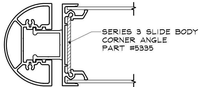
3/8" REVEAL POSITION
