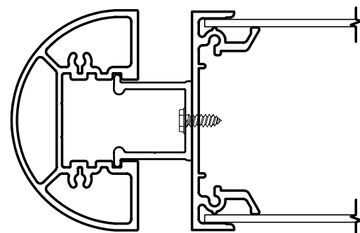
3/4" REVEAL POSITION
